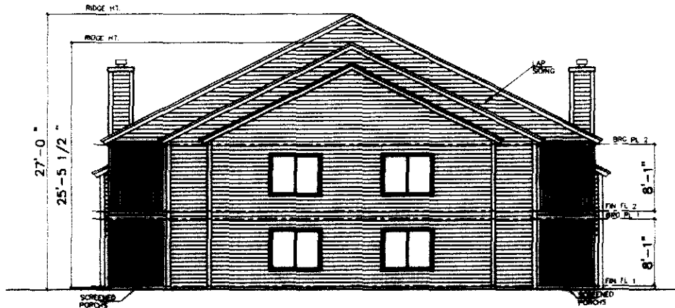
2 LEFT ELEVATION 3 BEDROOM UNIT BUILDING # 277
