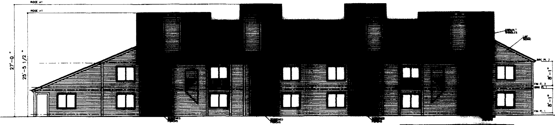
1 REAR ELEVATION ONE BEDROOM UNIT BUILDING # 275, 278
