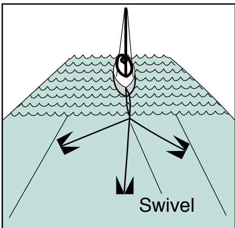
Using three anchors set 120° apart allows the boat to swing and face the wind. This is an especially good technique if the boat must be moored in a crowded harbor because the boat will not swing in as wide an arc as a boat that is riding on only two anchors.
